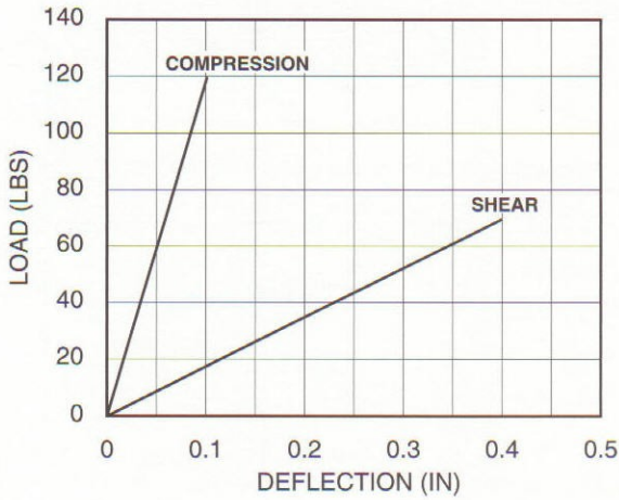
A32-151 Load vs Deflection
