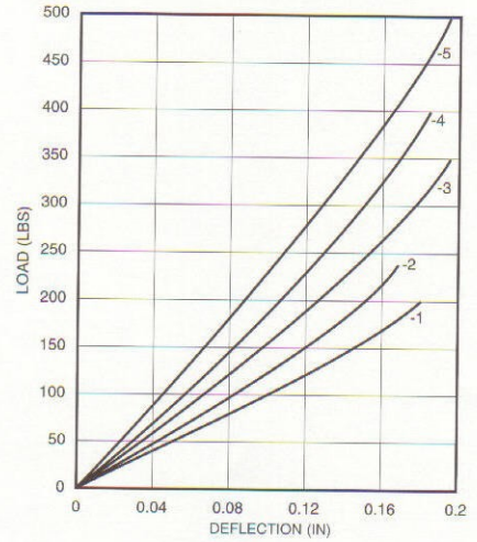
Load vs. Deflection
