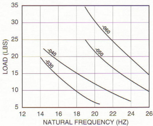
WR-3 Series Load vs Natural Frequency
