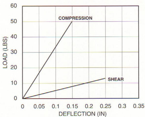
A23-141 Load vs Deflection
