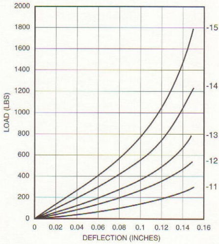
22001 Series Axial Load vs. Deflection
