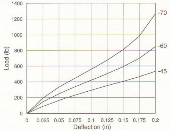
26748 Series - Axial Load vs. Deflection
