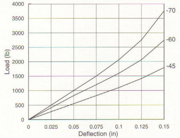
26748 Series - Radial Load vs. Deflection
