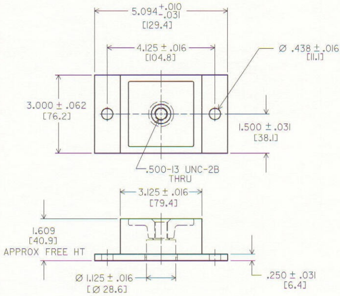
670 SERIES Dimensional Drawing
