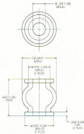
275 Series Dimensional Drawing
